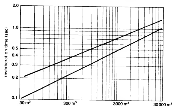
⑥ Reverberation time with respect to room volume
